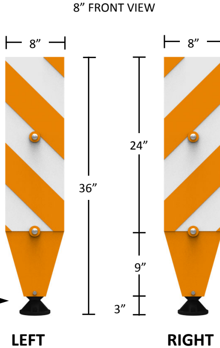
Reactive Unit
